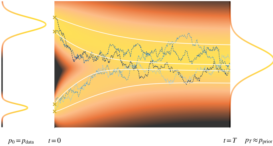
Figure 4.3: (1D) Visualization of the forward process in a diffusion model. The process starts from initial points sampled (denoted as “ \times ”) from a complex bimodal data distribution ( p_0 = p_{\text{data}} ) and evolves toward a simple, unimodal Gaussian prior ( p_T \approx p_{\text{prior}} ). The background heatmap illustrates the evolving marginal probability density, p_t , which smooths over time. Sample trajectories are shown evolving from t = 0 to t = T , comparing the stochastic forward SDE process (blue paths) with its deterministic counterpart, the PF-ODE (white paths). Note that the PF-ODE is a deterministic transport map for densities, not generally the mean of sample paths started from a single point.
